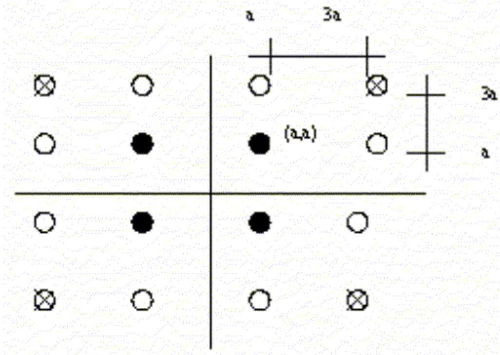
Fig.4. QAM constellations.
