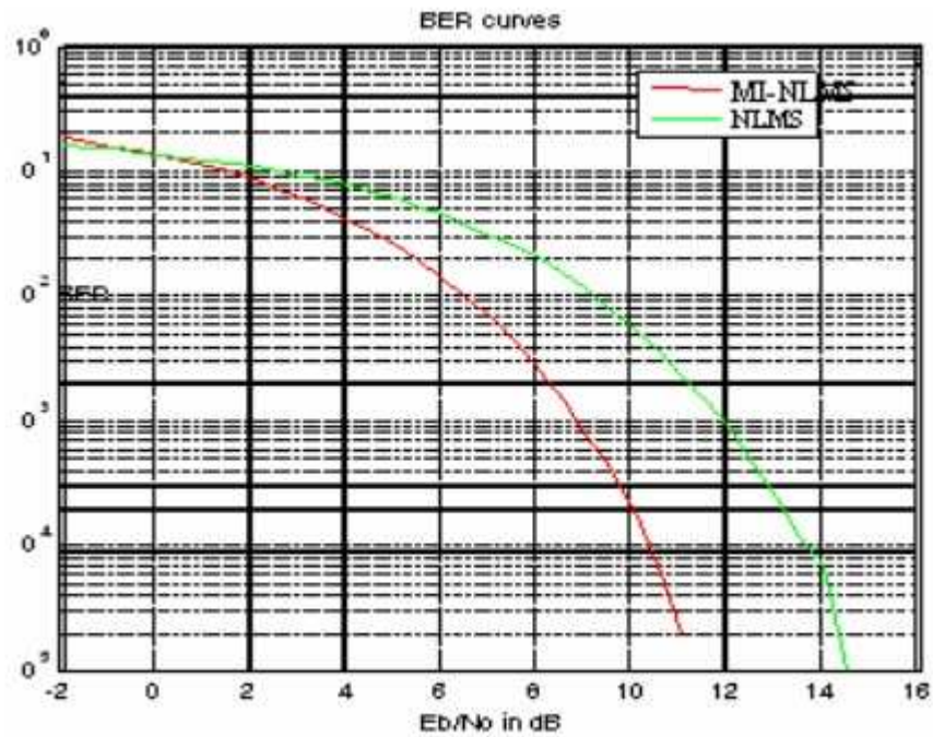
Figure .9. BER for 16-QAM.
