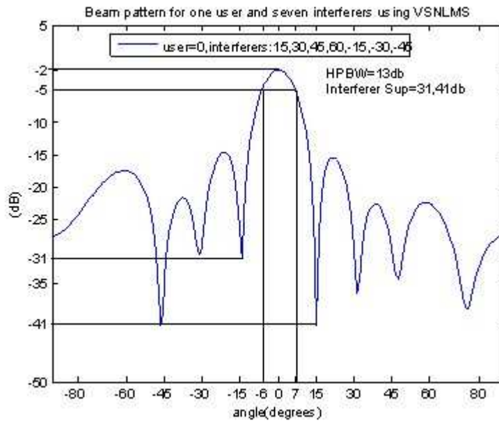
Figure.6.Beam pattern using NLMS.
