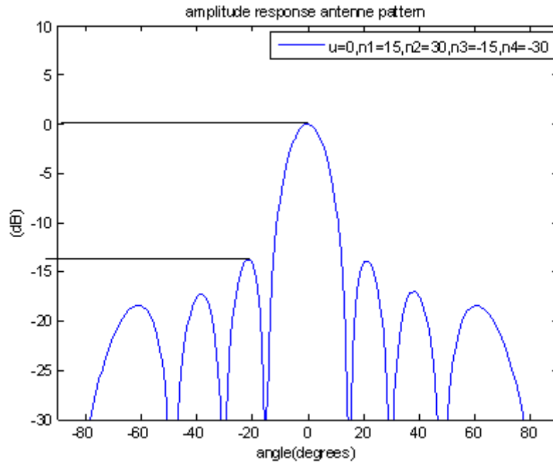
Figure 8 Array pattern with four interferers.
