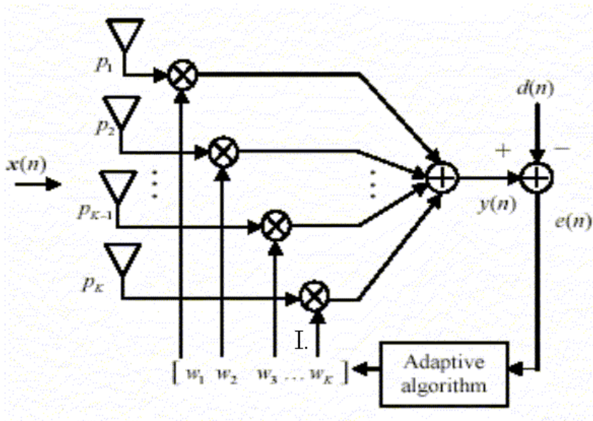
Figure.3. Block diagram of Adaptive beamforming
